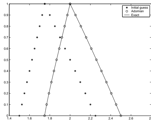
Fig. 2. Approximate and analytical solution of example (5.1) for y \geq 0 .
