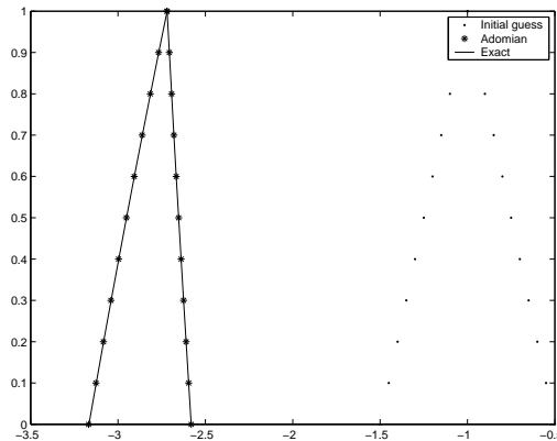
Fig. 6. Approximate and analytical solution of example (5.2) for y .
