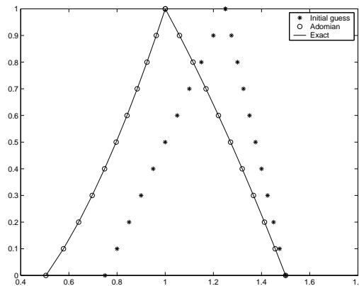
Fig. 1. Approximate and analytical solution of example (5.1) for x \geq 0 .
