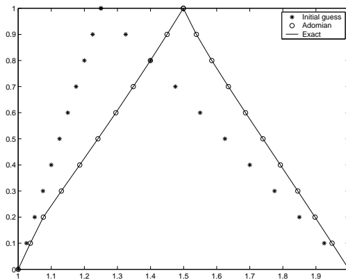
Fig. 4. Approximate and analytical solution of example (5.1) for y \leq 0 .
