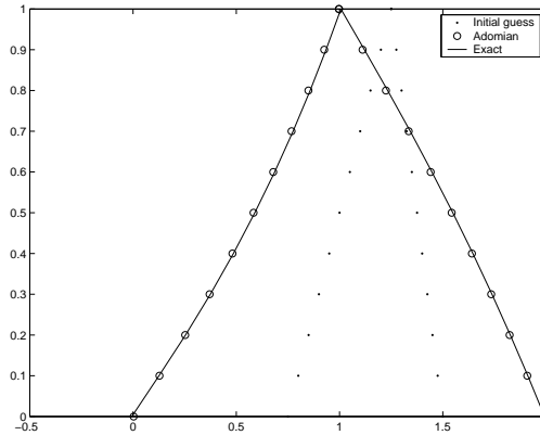
Fig. 7. Approximate and analytical solution of example (5.3) for x \geq 0 .
