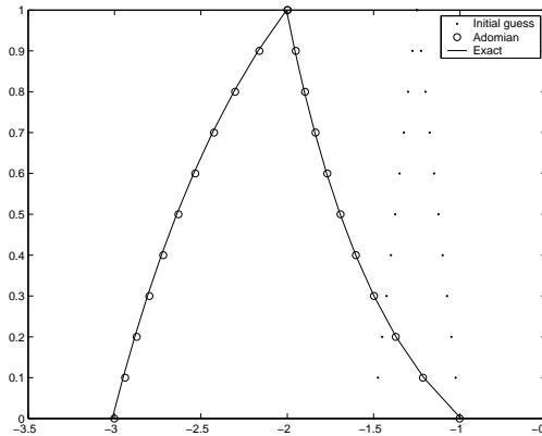
Fig. 8. Approximate and analytical solution of example (5.3) for y \leq 0 .
