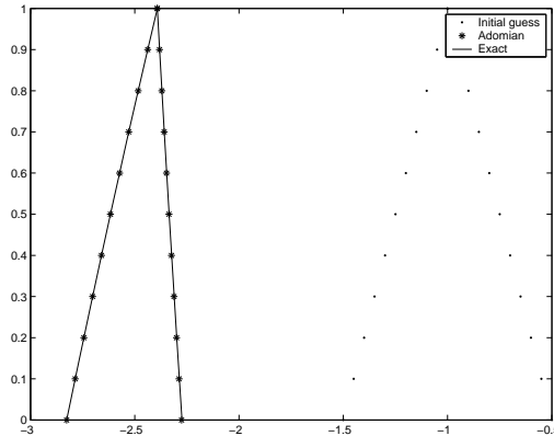
Fig. 5. Approximate and analytical solution of example (5.2) for x .
